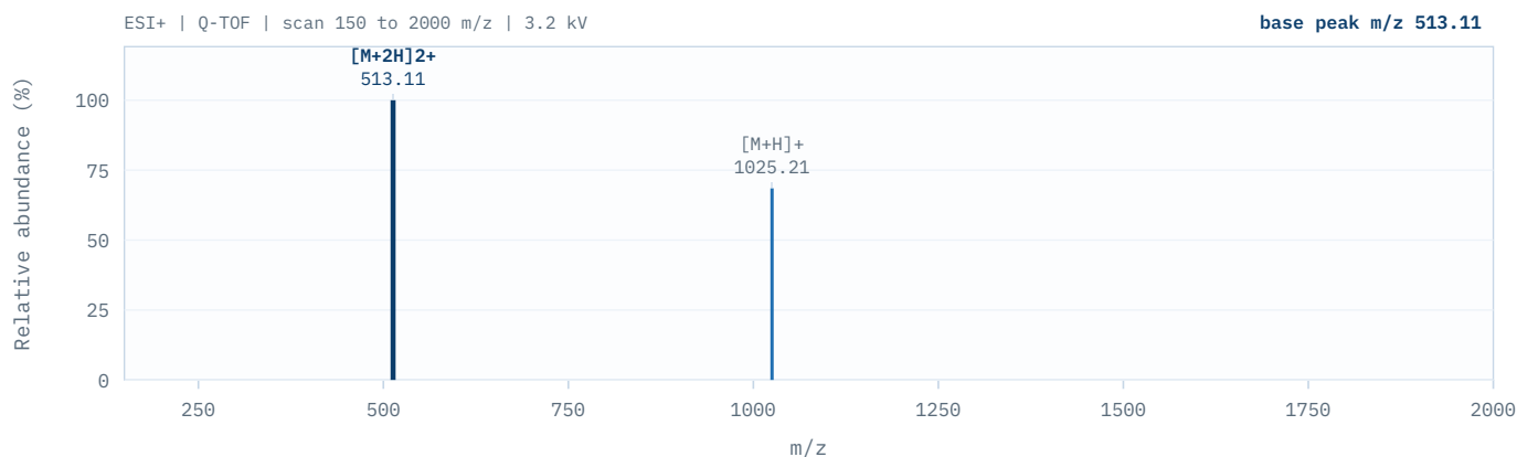
Figure 3. Theoretical ESI(+) charge-state ladder computed from 1024.20 Da. Replace with the acquired spectrum before issue.
